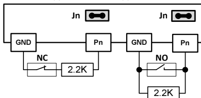
EOL mode (A3Y)
