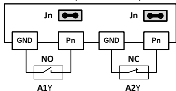
Without end of line resistor
